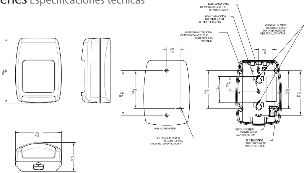
5800PIR WIRELESS MOTION SENSOR
