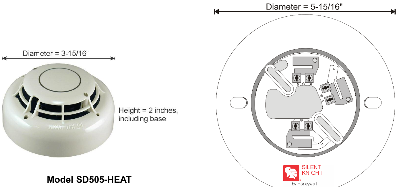
Model SD505-6AB Detector Base (Top View)
