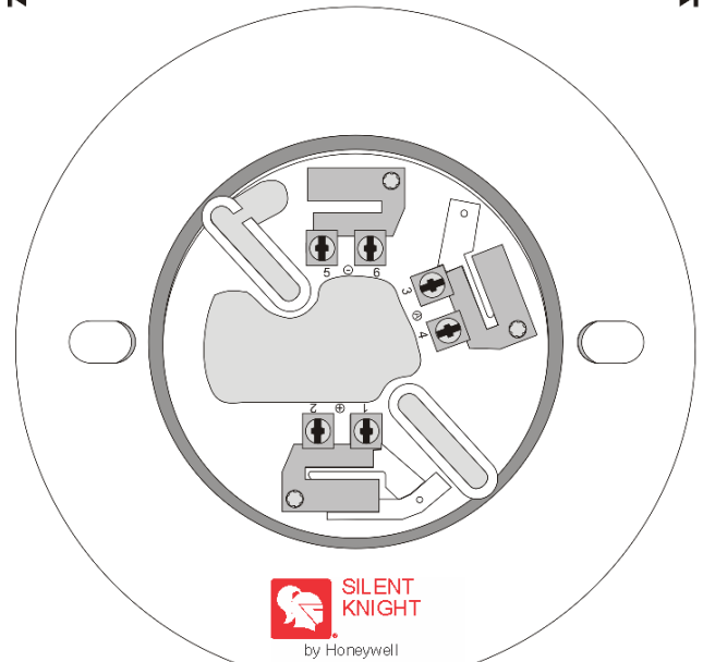
Model SD505-6AB Detector Base (Top View)
